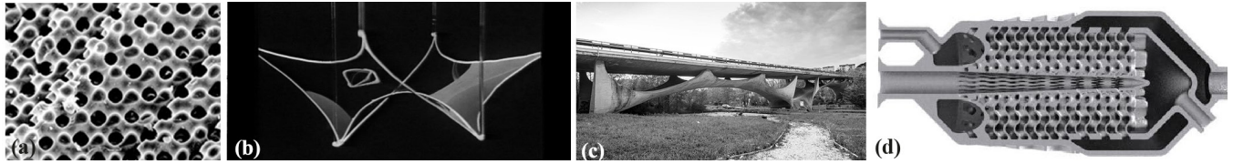
1 Shellular structures in nature, architecture and engineering; (a) cross-section through a sea urchin skeletal plate (Lai et al 2007), (b) Frei otto's physical form-finding using soap film (Otto 1970); (c) The bridge over the Basento by Sergio Musmeci (Canestrini, 1975); (d) Shellular structure's application in an aerospace turbine engine (Vlahinos and O'Hara 2020).
