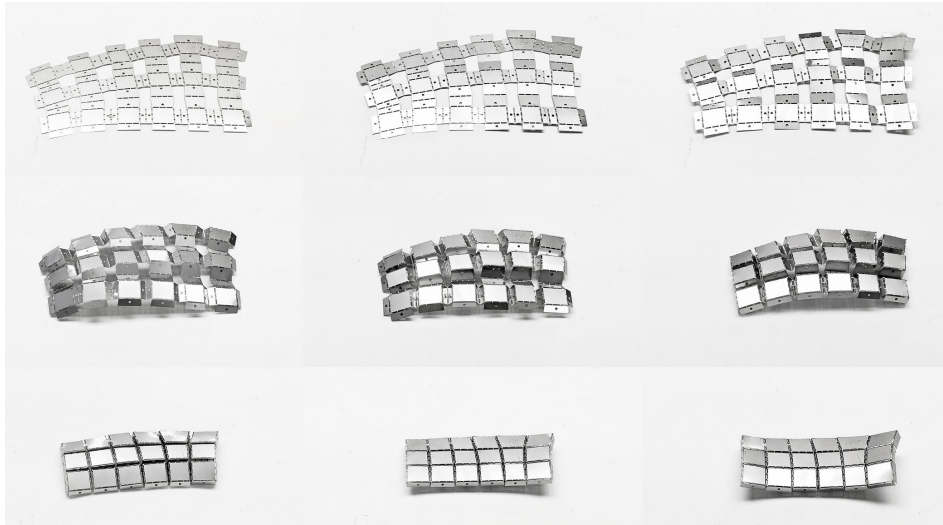
15 Folding a stainless steel sheet with different design parameters of dash line cuts.
